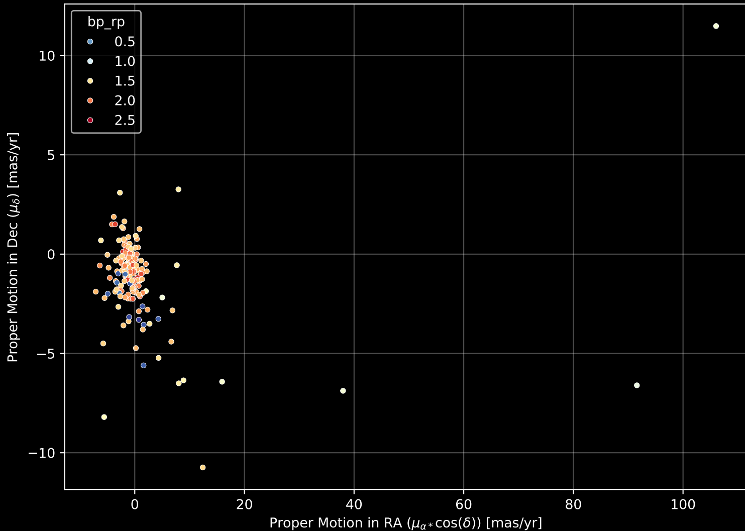
APOGEE DR17 Field: [128-04] Proper Motion Diagram (n= 182)
