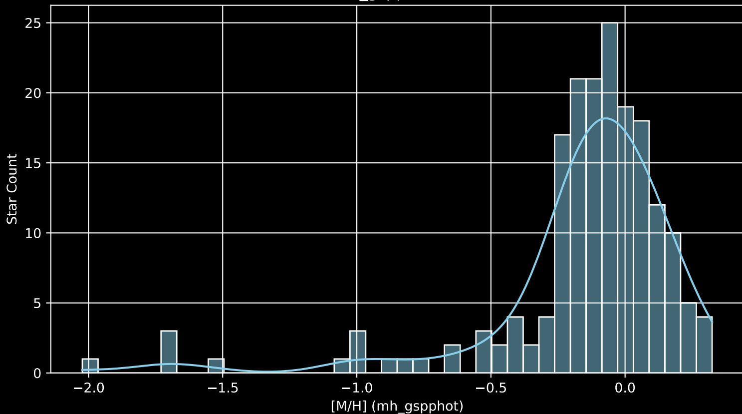
APOGEE DR17 Field: [128-04 [M/H] (mh_gspphot) (n= 181)
