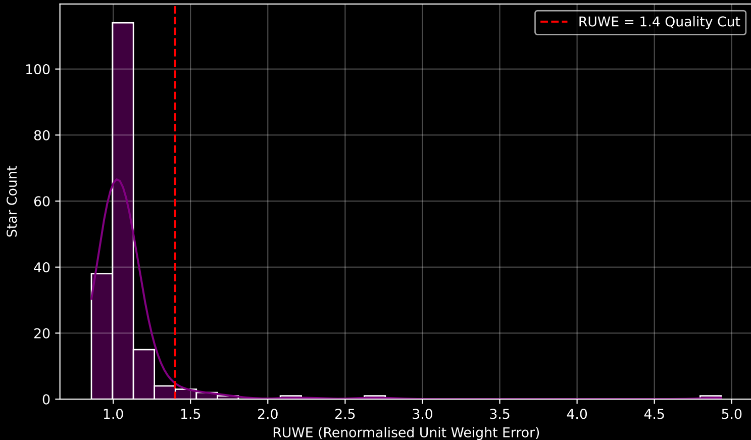
GAPOGEE DR17 Field [128-04] RUWE Distribution (n= 180)
