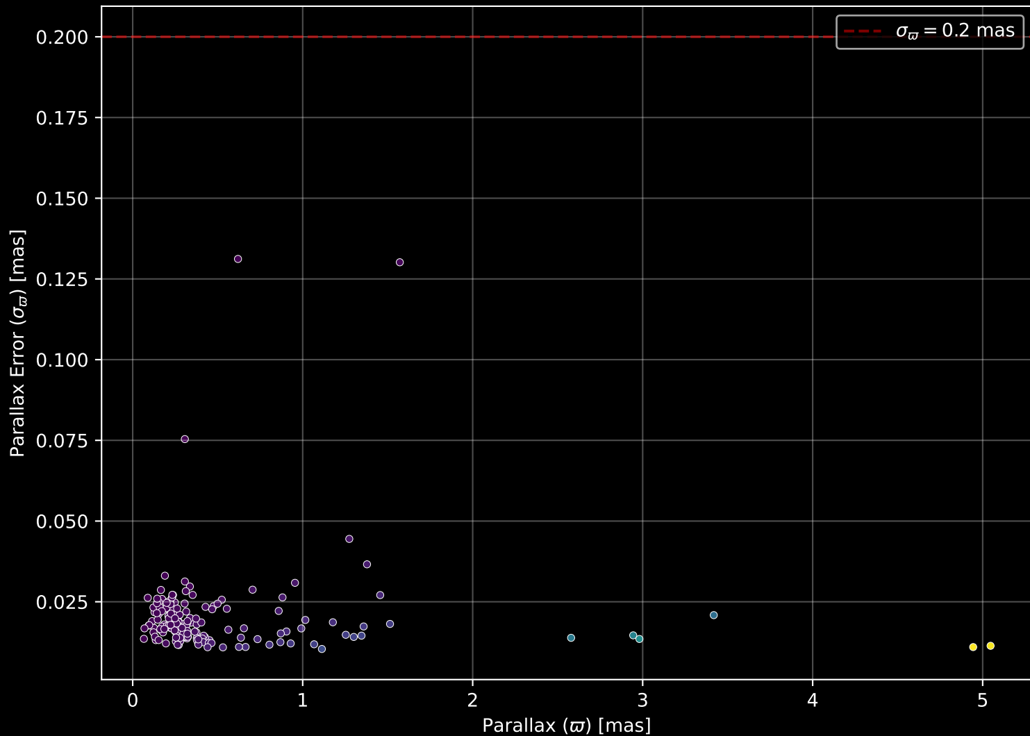
APOGEE DR17 Field: [128-04] Parallax Quality (n= 182)
